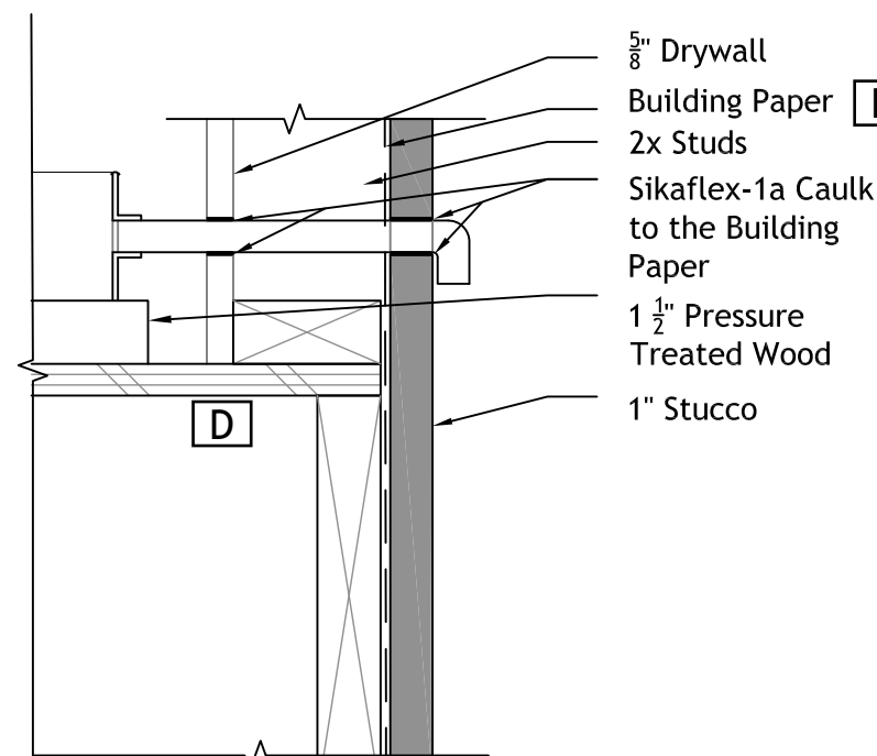
③ Stucco Wall Detail
