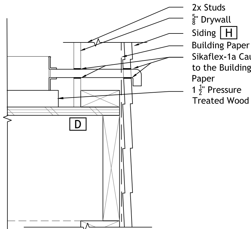
③ Siding Wall Detail
